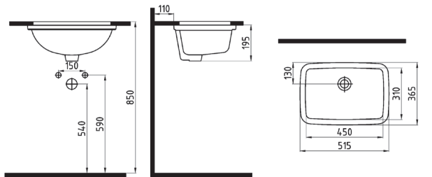
TEK PARÇA TEZGAH ALTI LAVABO BATARYA DELİKSİZ TPLA04501VDOW5000 45 cm
