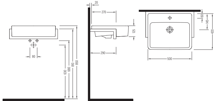
YARIM TEZGAH LAVABO DİKDÖRTGEN BATARYA DELİKLİ ROLY05003FD1W5000 500x420 mm
