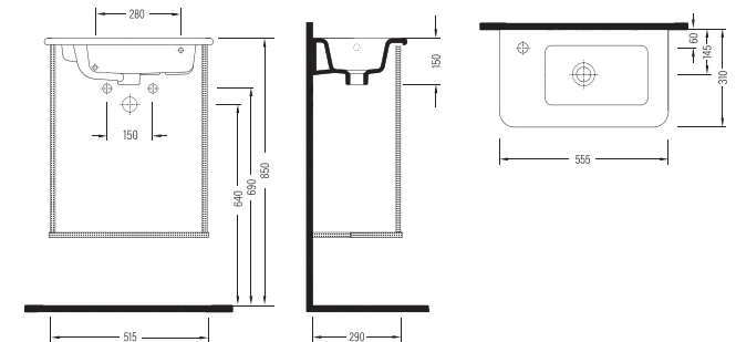
MOBİLYA UYUMLU LAVABO SOLDAN BATARYA DELİKLİ KSLKL55B1FD1W5000 555x310mm
