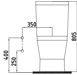
DUVARA SIFIR KLOZET TAKIMI BOX-RIM NPKD06301VP1W5000 630x350mm
