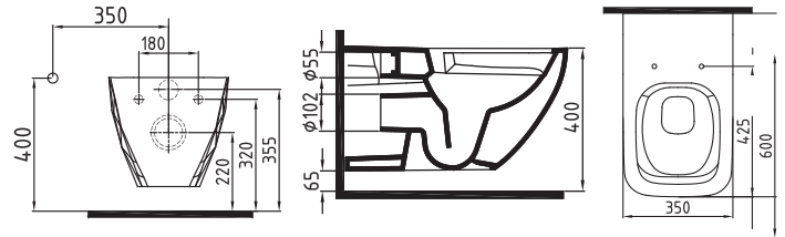
ASMA KLOZET NO-RIM KRKA060N1VP1W5000 600x350mm
