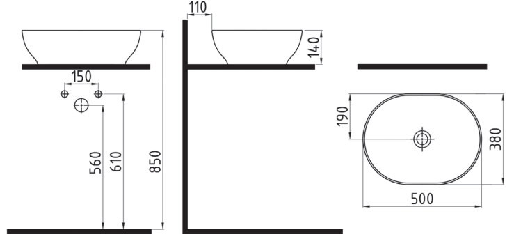
OBLONG TEZGAH ÜSTÜ LAVABO BATARYA DELİKSİZ MTLG05001FDOW5000 500x380mm
