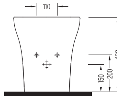
DUVARA SIFIR BİDE ROBY05201VD1W5000 520x355 mm
