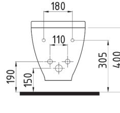
ASMA BİDE HRBA05201VD1W5000 520x350mm
