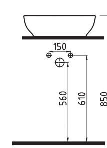
ASİMETRİK TEZGAH ÜSTÜ LAVABO BATARYA DELİKSİZ MTLG05004FDOW5000 500x380mm
