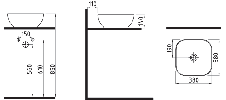
KARE TEZGAH ÜSTÜ LAVABO BATARYA DELİKSİZ MTLG03801FDOW5000 380x380mm
