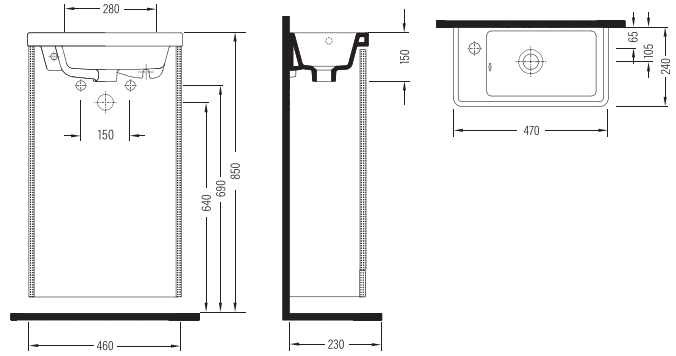
MOBİLYA UYUMLU LAVABO SOLDAN BATARYA DELİKLİ KSLK047B1FD1W5000 470x240mm
