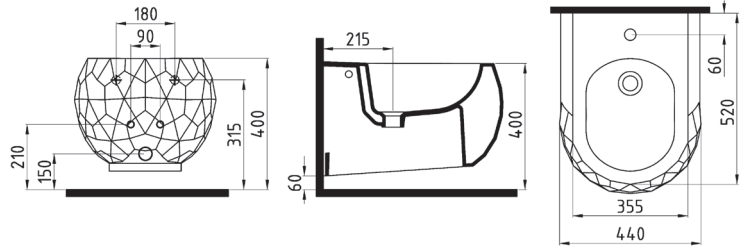
ASMA BİDE PNBA05201VD1W5000 520x355mm
