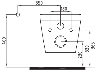
ASMA KLOZET NO-RIM NPKA052N1VP1W5000 520x350mm
