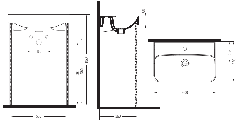
MOBİLYA UYUMLU LAVABO BATARYA DELİKLİ ROLK060B1FD1W5000 600x380 mm
