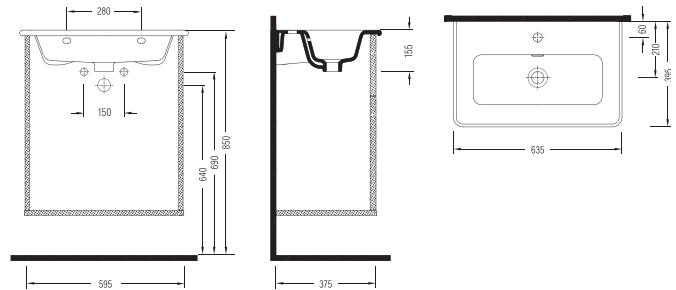
MOBİLYA UYUMLU LAVABO BATARYA DELİKLİ KSLK063B1FD1W5000 635x395mm
