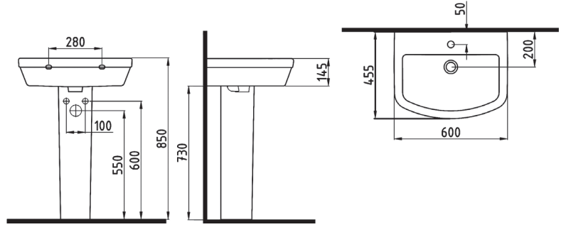
DUVARA MONTAJLI LAVABO BATARYA DELİKLİ DRLS06001VD1W5000 600x455mm
