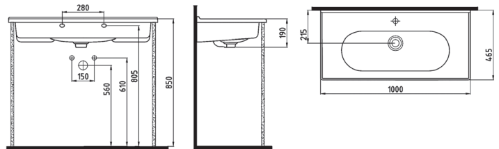
MOBİLYA UYUMLU LAVABO BATARYA DELİKLİ FELK10001FD1W5000 1000x465mm
