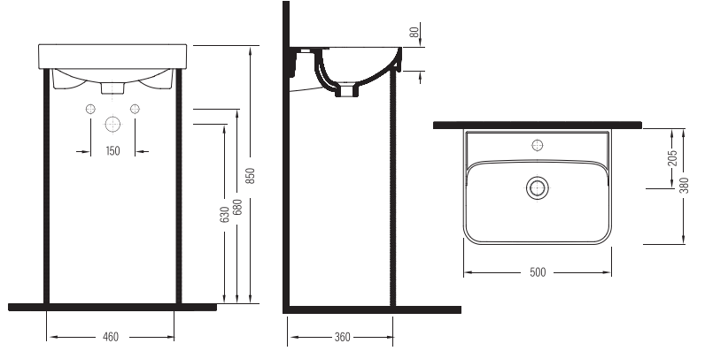
MOBİLYA UYUMLU LAVABO BATARYA DELİKLİ ROLK050B1FD1W5000 500x380 mm
