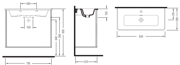
MOBİLYA UYUMLU LAVABO BATARYA DELİKLİ KSLK083B1FD1W5000 830x395mm
