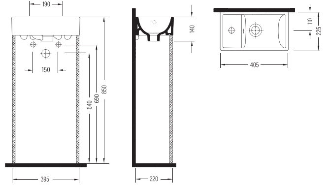
TEZGAH ÜSTÜ LAVABO SOLDAN BATARYA DELİKLİ KSLGL40B1FD1W5000 405x225mm
