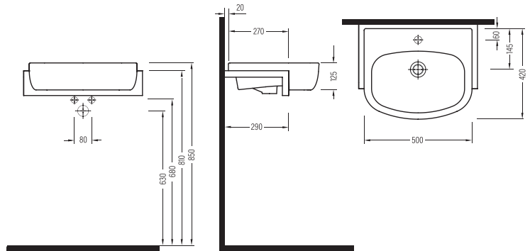
YARIM TEZGAH LAVABO OVAL BATARYA DELİKLİ ROLY05001FD1W5000 500x420 mm
