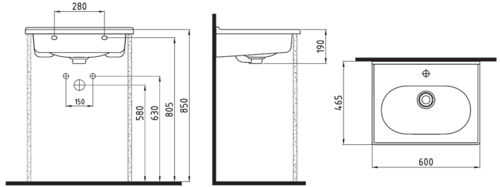
MOBİLYA UYUMLU LAVABO BATARYA DELİKLİ FELK060B1FD1W5000 600x465mm
