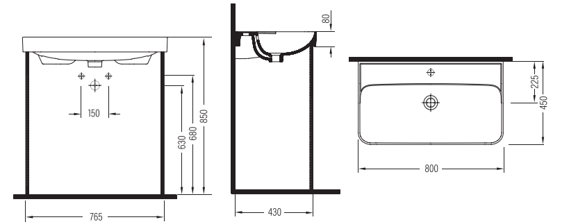
MOBİLYA UYUMLU LAVABO BATARYA DELİKLİ ROLK080B1FD1W5000 800x450 mm
