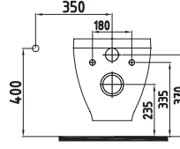
ASMA KLOZET BOX-RIM HRKA052AMVP1W5000 520x350mm
