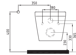
ASMA KLOZET BOX-RIM NPKA052AMVP1W5000 520x350mm
