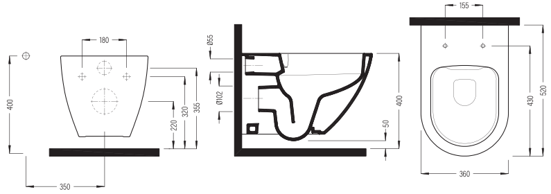
ASMA KLOZET NO-RIM NCKA052H1VP1W5000 520x360 mm
