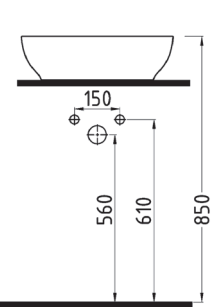
DİKDÖRTGEN TEZGAH ÜSTÜ LAVABO BATARYA DELİKSİZ MTLG05003FDOW5000 495x380mm
