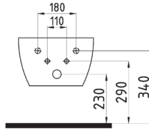
N3 ASMA BİDE HRBA05203VD1W5000 530x350mm
