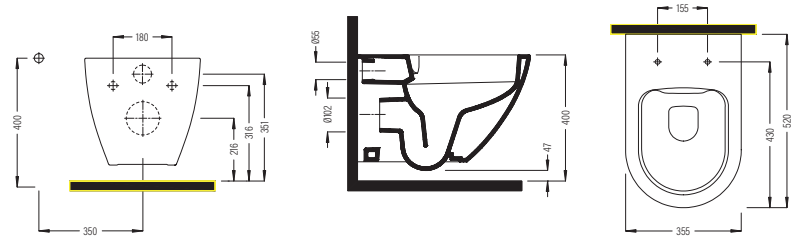
ASMA KLOZET NO-RIM NCKA052N1VP1W5000 520x355 mm
