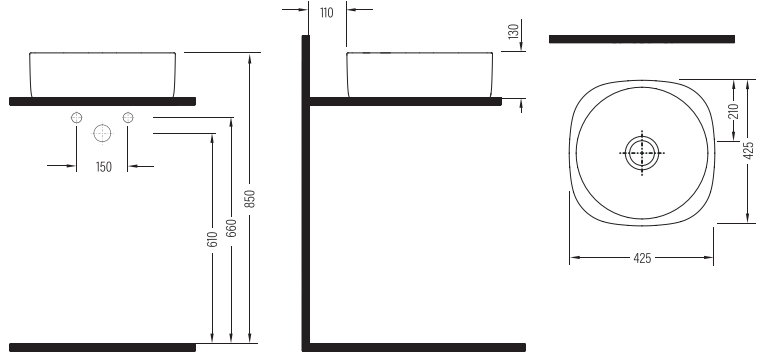
TEZGAH ÜSTÜ LAVABO BATARYA DELİKSİZ SQLG04301FD0W5000 425x425 mm
