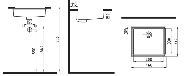
INFINITUM TEZGAH ALTI LAVABO BATARYA DELİKSİZ INLA04001FDOW5000 40 cm
