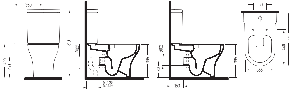
OVAL DUVARA SIFIR KLOZET TAKIMI NO-RIM ROKD063N1VP1W5000 620x355 mm
