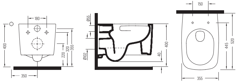
ASMA KLOZET VORTEX SQKA052V1VP1W5000 520x355 mm
