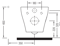
ASMA KLOZET VORTEX SOKA052V1VP1W5000 520x360 mm
