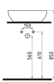
OVAL TEZGAH ÜSTÜ LAVABO BATARYA DELİKSİZ MTLG05002FDOW5000 495x375mm
