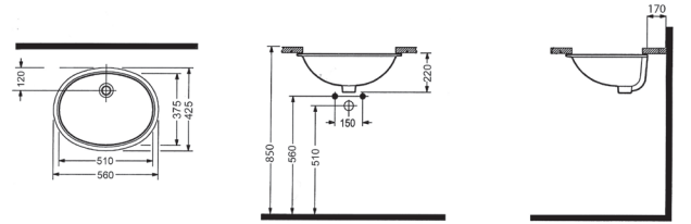
TEK PARÇA TEZGAH ALTI LAVABO BATARYA DELİKSİZ TPLA05001VDOW5000 50 cm
