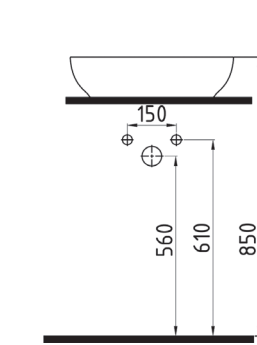
OVAL TEZGAH ÜSTÜ LAVABO BATARYA DELİKLİ MTLG05005FD1W5000 500x380mm
