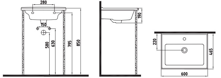
MOBİLYA UYUMLU LAVABO BATARYA DELİKLİ NPLK06001FD1W5000 600x470mm
