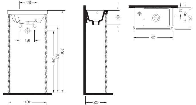
MOBİLYA UYUMLU LAVABO SOLDAN BATARYA DELİKLİ KSLKL41B1FD1W5000 410x225mm
