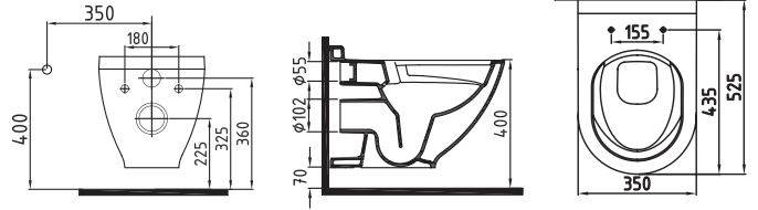
N5 ASMA KLOZET NO-RİM HRKA052N5VP1W5000 525x350mm
