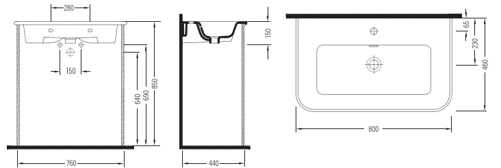
MOBİLYA UYUMLU LAVABO BATARYA DELİKLİ KSLK080B1FD1W5000 800x460mm
