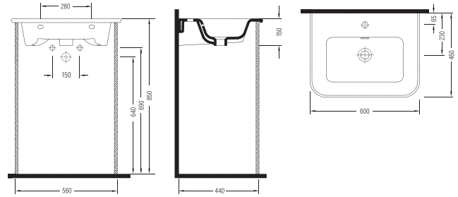
MOBİLYA UYUMLU LAVABO BATARYA DELİKLİ KSLK060B1FD1W5000 600x460mm
