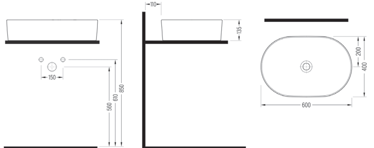
OBLONG TEZGAH ÜSTÜ LAVABO SOLG060S1FD0W5000 600x400 mm
