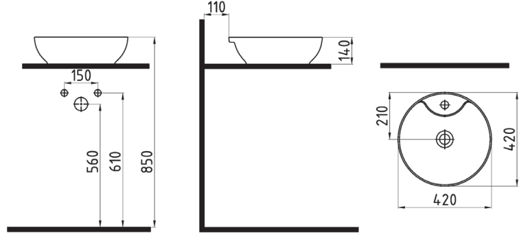
YUVARLAK TEZGAH ÜSTÜ LAVABO BATARYA DELİKLİ MTLG04202FD1W5000 420x420mm
