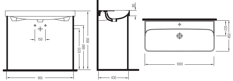
MOBİLYA UYUMLU LAVABO BATARYA DELİKLİ ROLK19001FD1W5000 1000x450 mm
