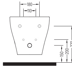
ASMA BİDE ROBA05001VD1W5000 500x355 mm
