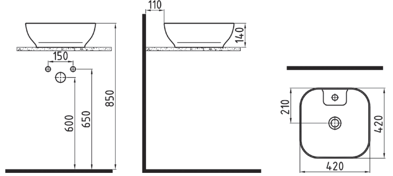
KARE TEZGAH ÜSTÜ LAVABO BATARYA DELİKLİ MTLG04201FD1W5000 420x420mm
