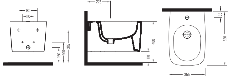
ASMA BİDE SQBA05201VD1W5000 520x355 mm
