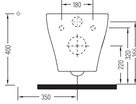
ASMA KLOZET NO-RIM ROKA050N1VP1W5000 500x360 mm
