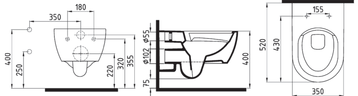
N3 ASMA KLOZET NO-RİM HRKA052N3VP1W5000 520x350mm
