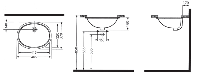
TEK PARÇA TEZGAH ALTI LAVABO BATARYA DELİKSİZ TPLA04101VDOW5000 41 cm
