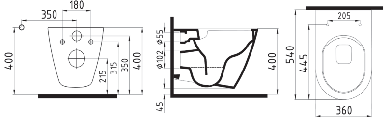
ASMA KLOZET NO-RIM ALKA054N1VP1W5000 540x360mm
