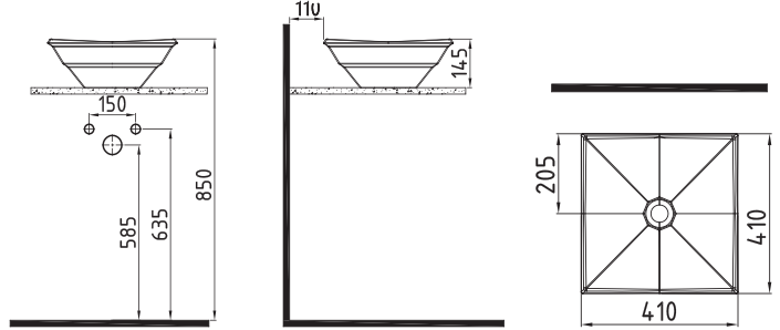
TEZGAH ÜSTÜ LAVABO KRLG04101FDOW5000 410x410mm
